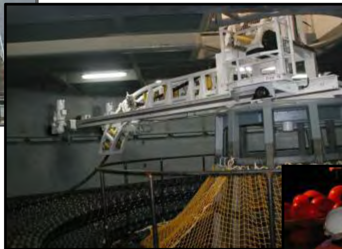
Loading/unloading arm in cable storage tank
